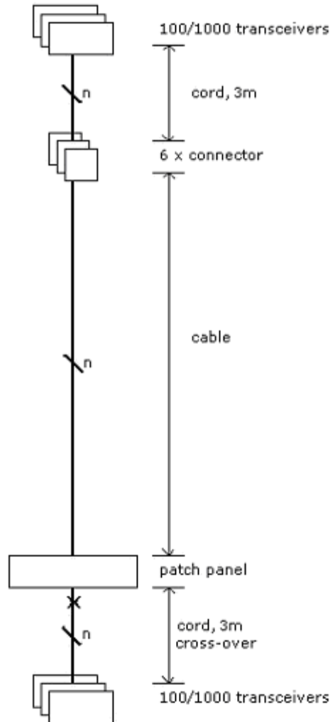
Figure 2-1 Channel Layout
