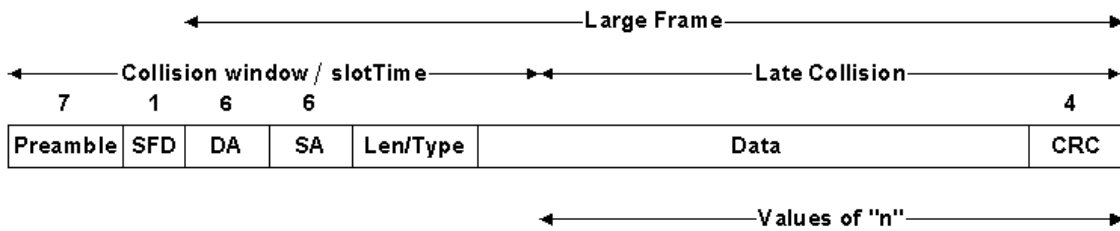
Figure 4 - 9 Collisions in data after slotTime
