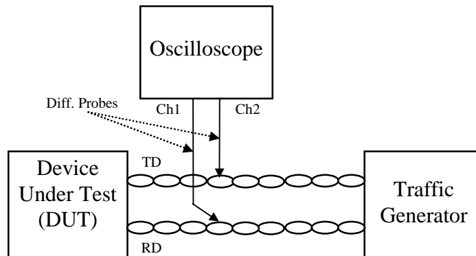
Figure 4 - 19 Test Setup for 10BASE-T Device
