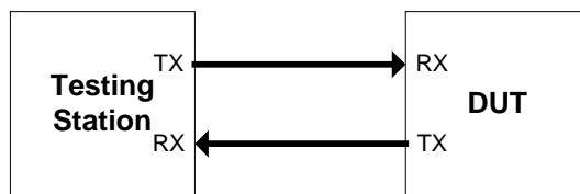
Figure 4 - 24 Test Setup for 1000BASE-T Devices
