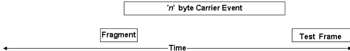
Figure 4 - 14 Deference after collision
