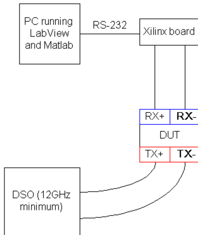
Figure 72.A-1: Setup #1 for performing startup tests
