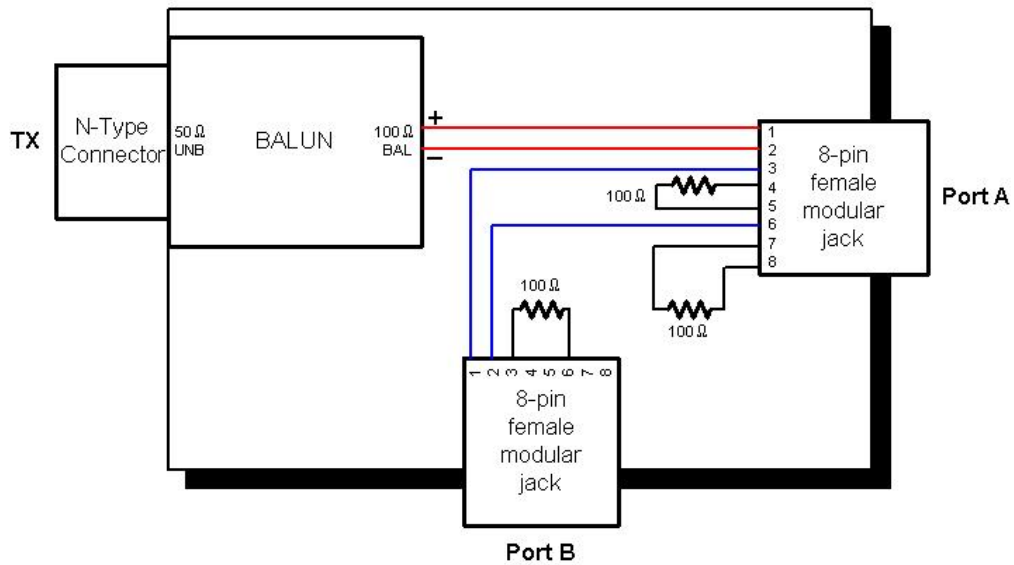
Figure 25.A-8: Test jig #2
