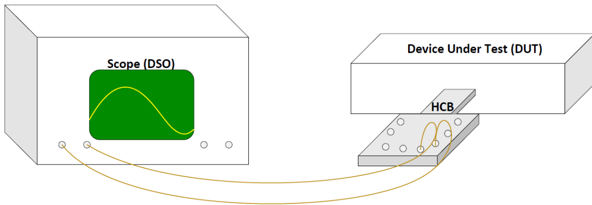
136.I – 1: Setup used for Group 1: Transmitter Electrical testing
