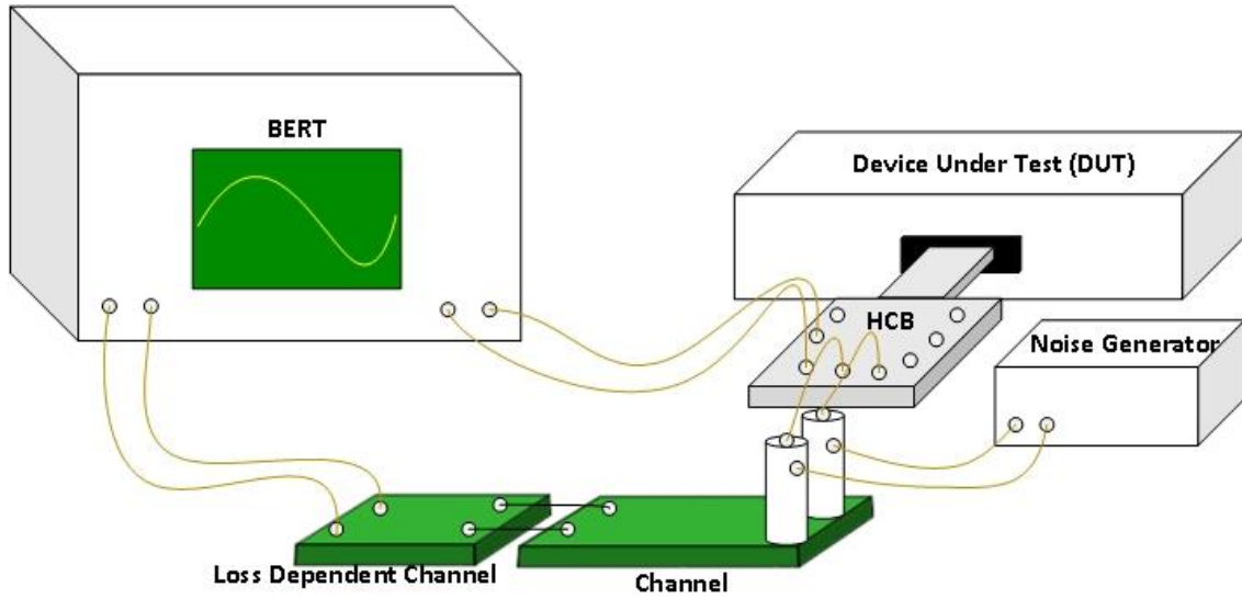
136.I – 3: Setup used for Group 4: Receiver Electrical Requirements testing
