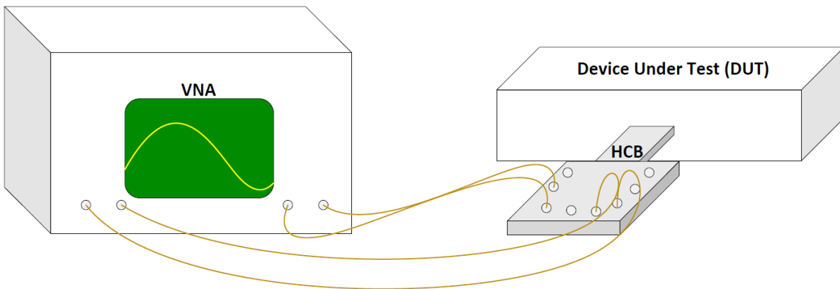
136.I – 2: Setup used for Group 3: Impedance Requirements testing
