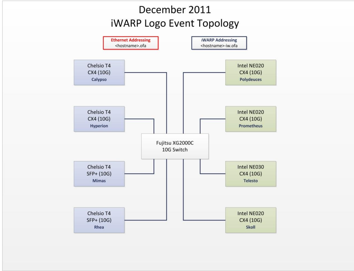
Figure 1: The IW fabric configuration utilized for all testing is shown below.
