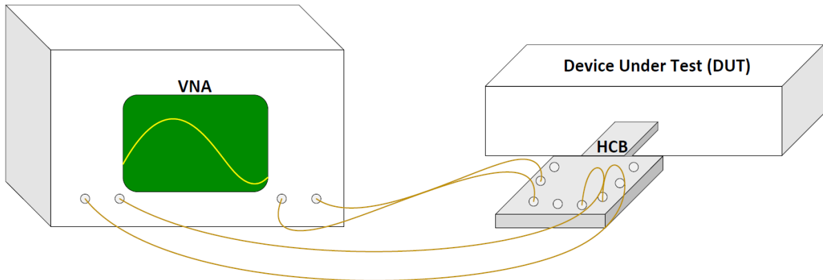
120.I – 2: Setup used for Group 3: Impedance Requirements testing
