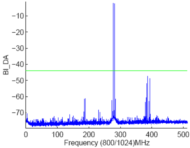
Figure 5: Linearity, Tone Pair #5
