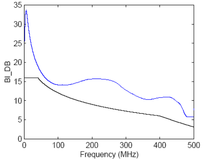
Figure 10: Return loss vs. frequency
