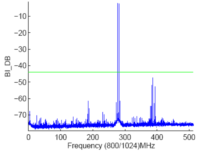
Figure 5: Linearity, Tone Pair #5
